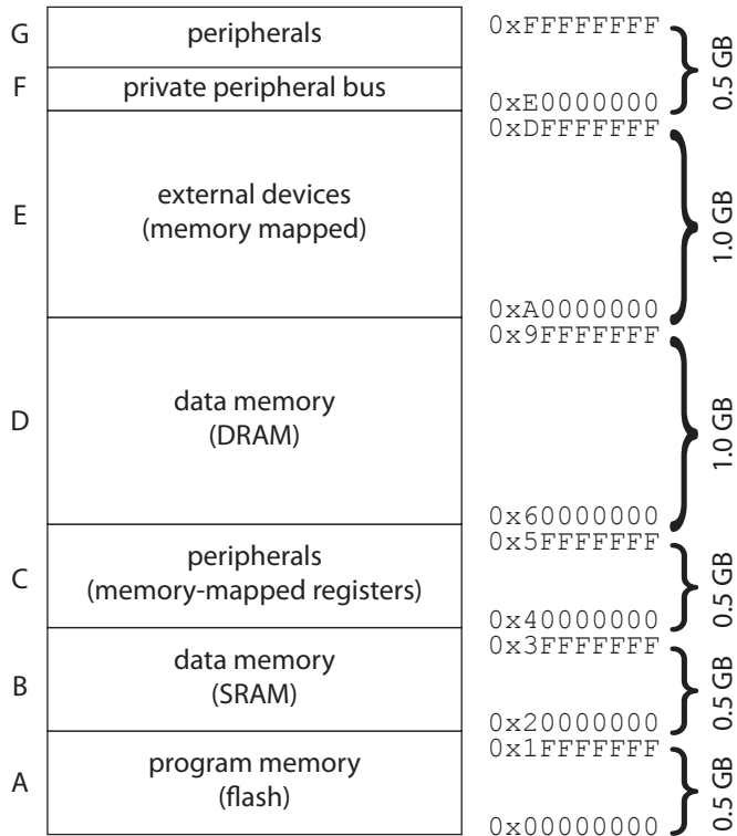
Figure 8.1: Memory map of an ARM Cortex TM - M3 architecture.
