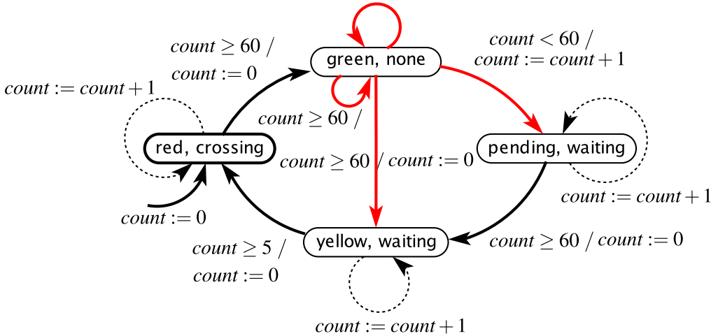
Figure 14.4: Extended state machine obtained from synchronous-reactive composition of traffic light controller and pedestrian models. Note that this is non-deterministic.
