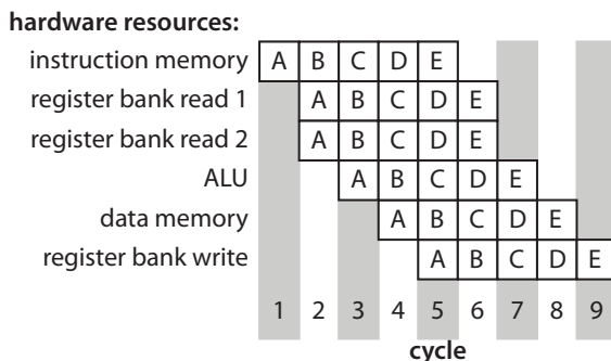
Figure 7.3: Reservation table for the pipeline shown in Figure 7.2.
